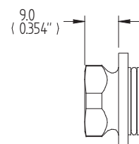
FF20-A 1/8" NPT Female Fitting
